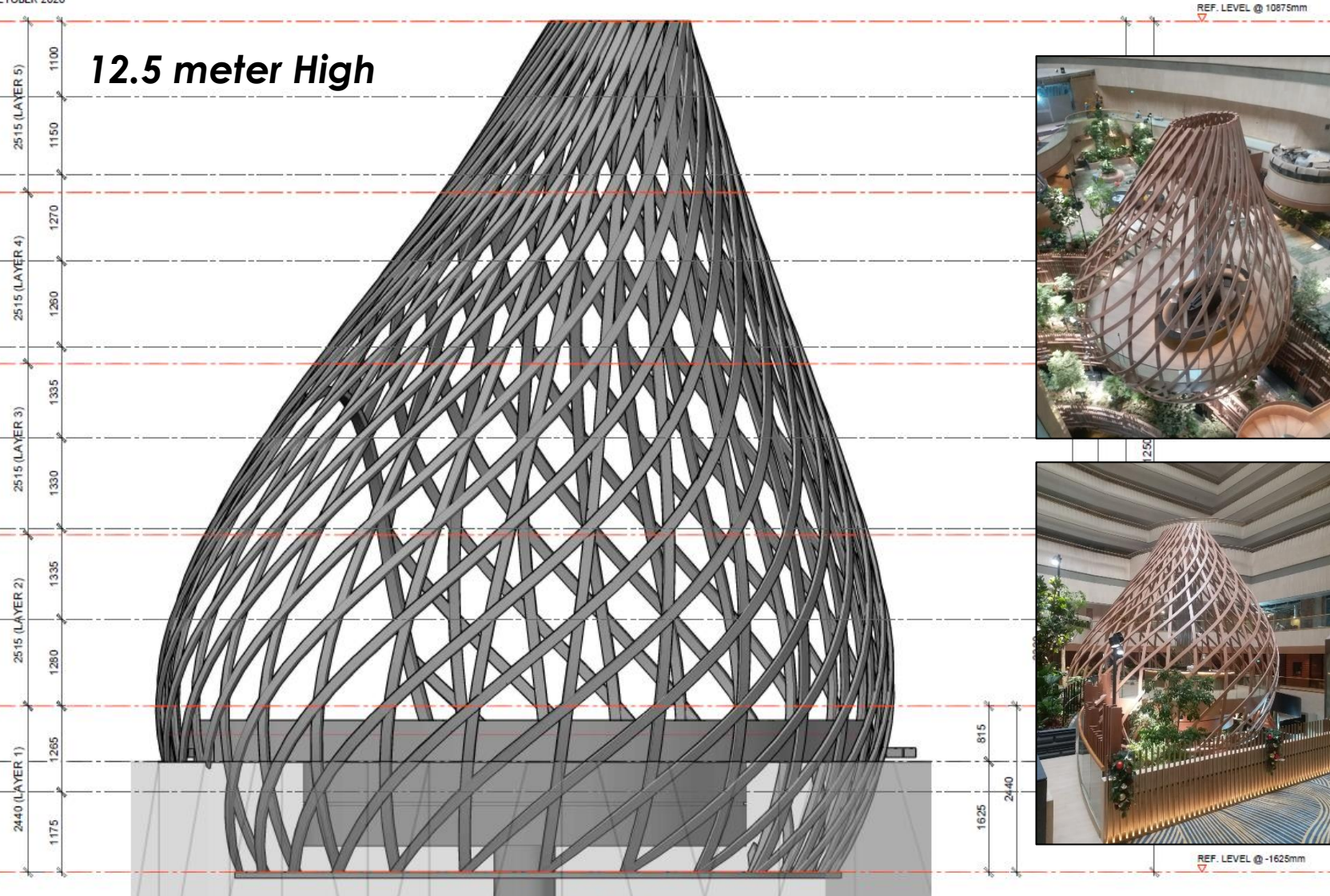
BAR POD_ELEVATION REFERENCE
